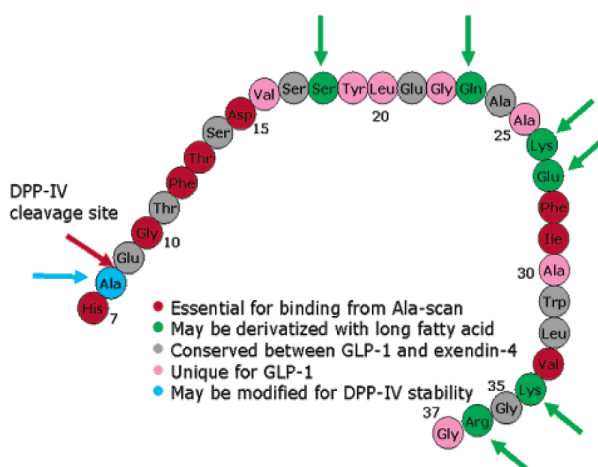
Figure 3. SAR figure of GLP-1. All sites essential for binding from Ala-scan are also conserved between GLP-1 and exendin-4. Sites that are possible to modify with fatty acids are only color-coded as such. They are all unique for GLP-1 at the same time.
